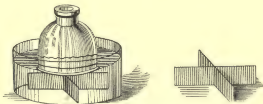
FIG. 49.—A second method of using Graham's bell dialyzer.
